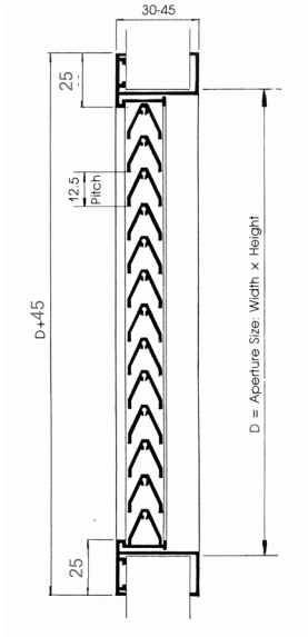
Non-Vision Transfer Grille DTG2
