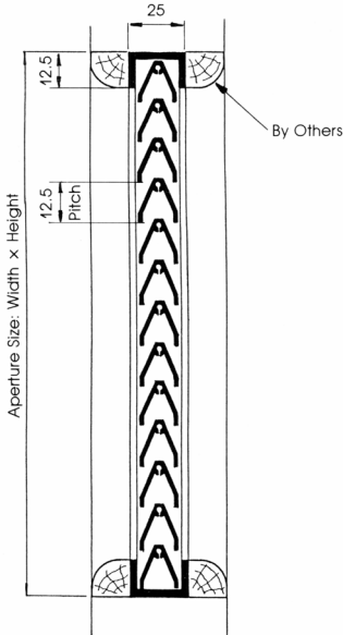
Non-Vision Transfer Grille Type DTG
