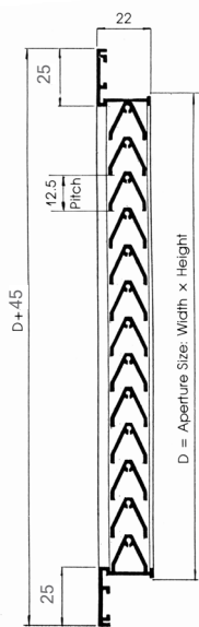
Non-Vision Transfer Grille Type DTG1
