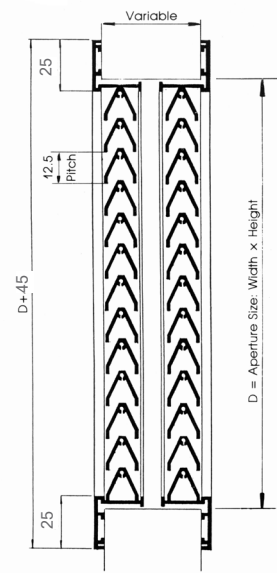
Non-Vision Transfer Grilles DTG1-2 Off
